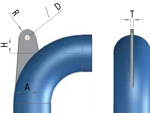
DİRSEK I PLAKASI / ELBOW EYE PLATE
