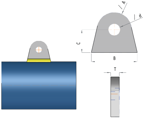
YATAY BORU I PLAKASI / HORIZONTAL PIPE EYE PLATE
