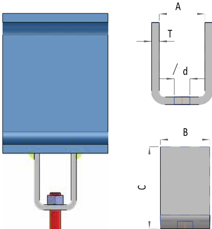
KİRİŞ U PLAKASI / BEAM U PLATE
