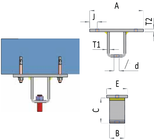
TAVAN TESPİT PLAKASI / CEILING FIXING PLATE
