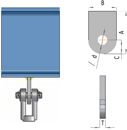
KİRİŞİ PLAKASI / BEAM EYE PLATE
