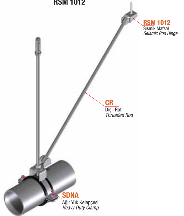
RSM 1012
