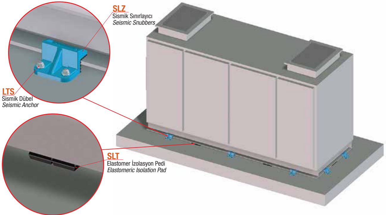
Klima Santrali Air Handling Unit
